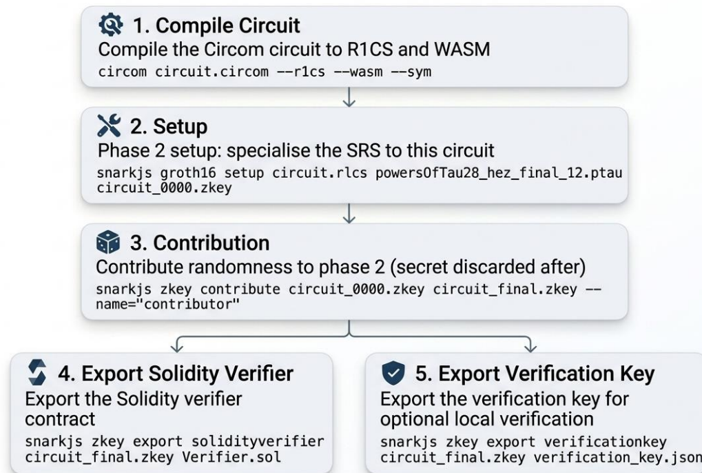
Figure 5.2 - Trusted Setup Two-Phase Pipeline (§5.4)
