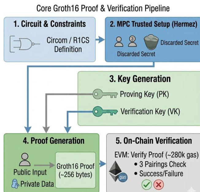
Figure 2.4 - Groth16 Proof Structure / Trusted Setup Pipeline (§2.3.3)
